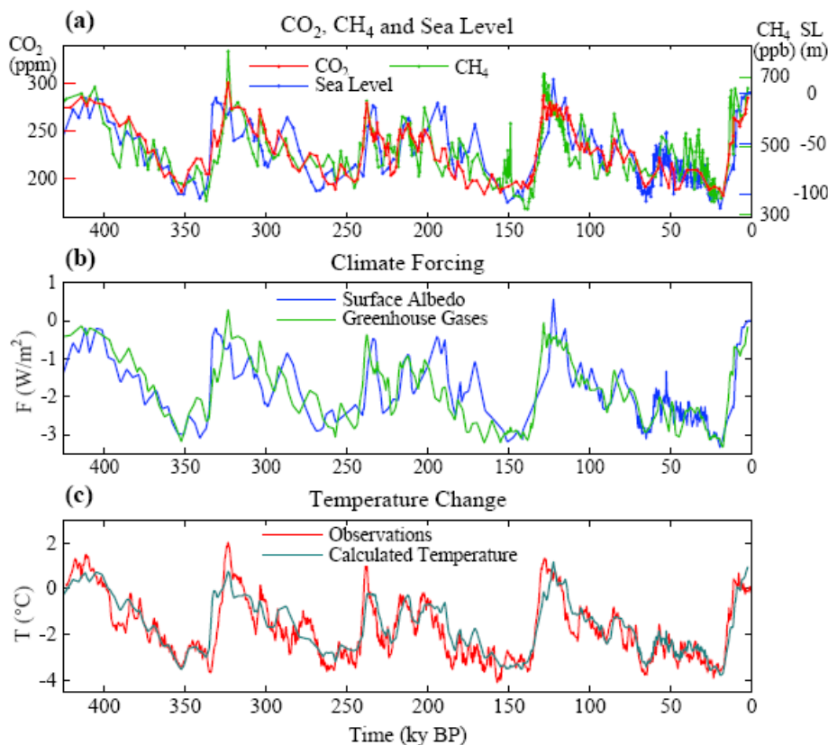
Fig. (1). (a) CO 2 , CH 4 [17] and sea level [19] for past 425 ky.
