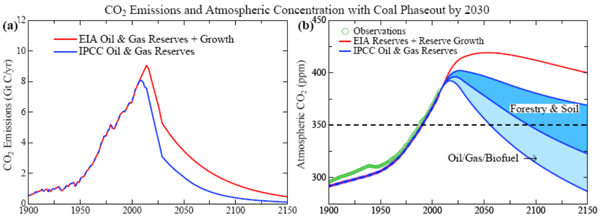
Fig. (6). (a) Fossil fuel CO 2 emissions with coal phase-out by 2030 based on IPCC [2] and EIA [80] estimated fossil fuel reserves. (b) Resulting atmospheric CO 2 based on use of a dynamic-sink pulse response function representation of the Bern carbon cycle model [78, 79].
